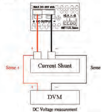
DC Voltage measurement
